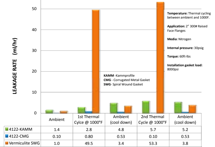
Leakage Test with Thermal Cycling (Metallic Gasket)
